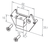
23 374.2101 16 x 16 mm, Zapfen 12 mm
