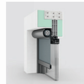
ZIP-Screen
